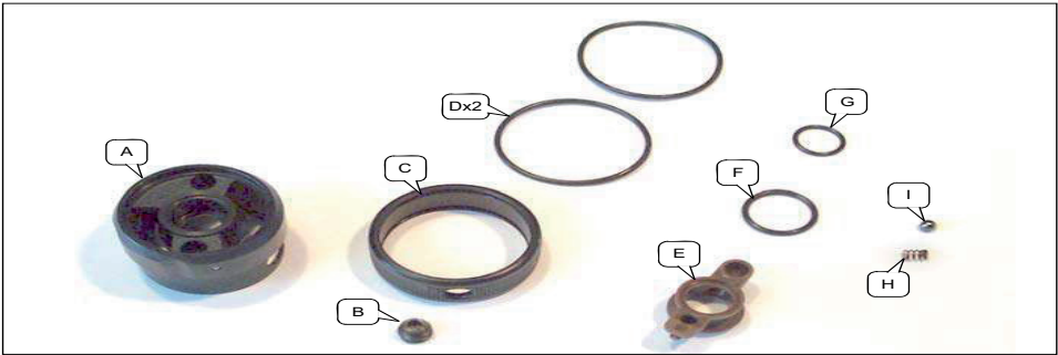
Reverse Housing Assembly
