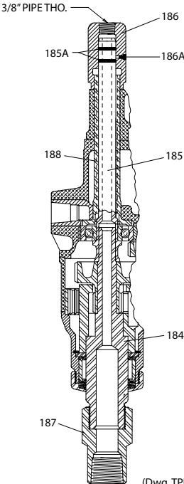
LEVER THROTTLE FOR DRILL WITH WATER ATTACHMENT
